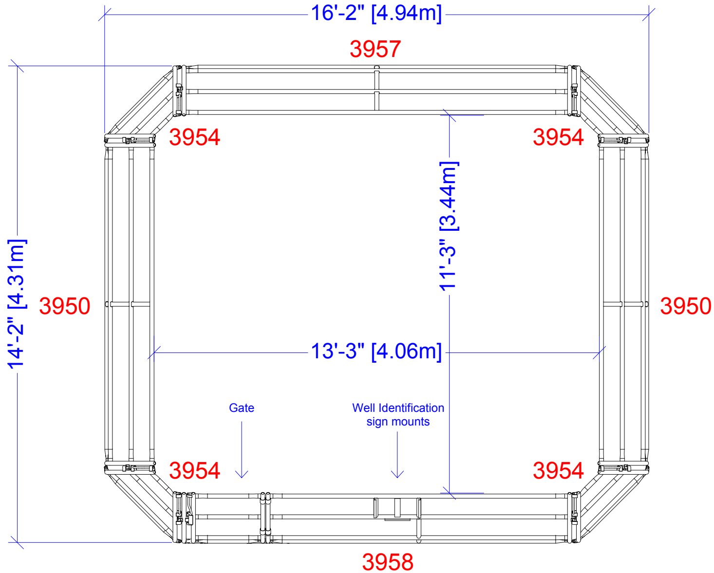
11'-3" x 13'-3" Wellfence Enclosure
