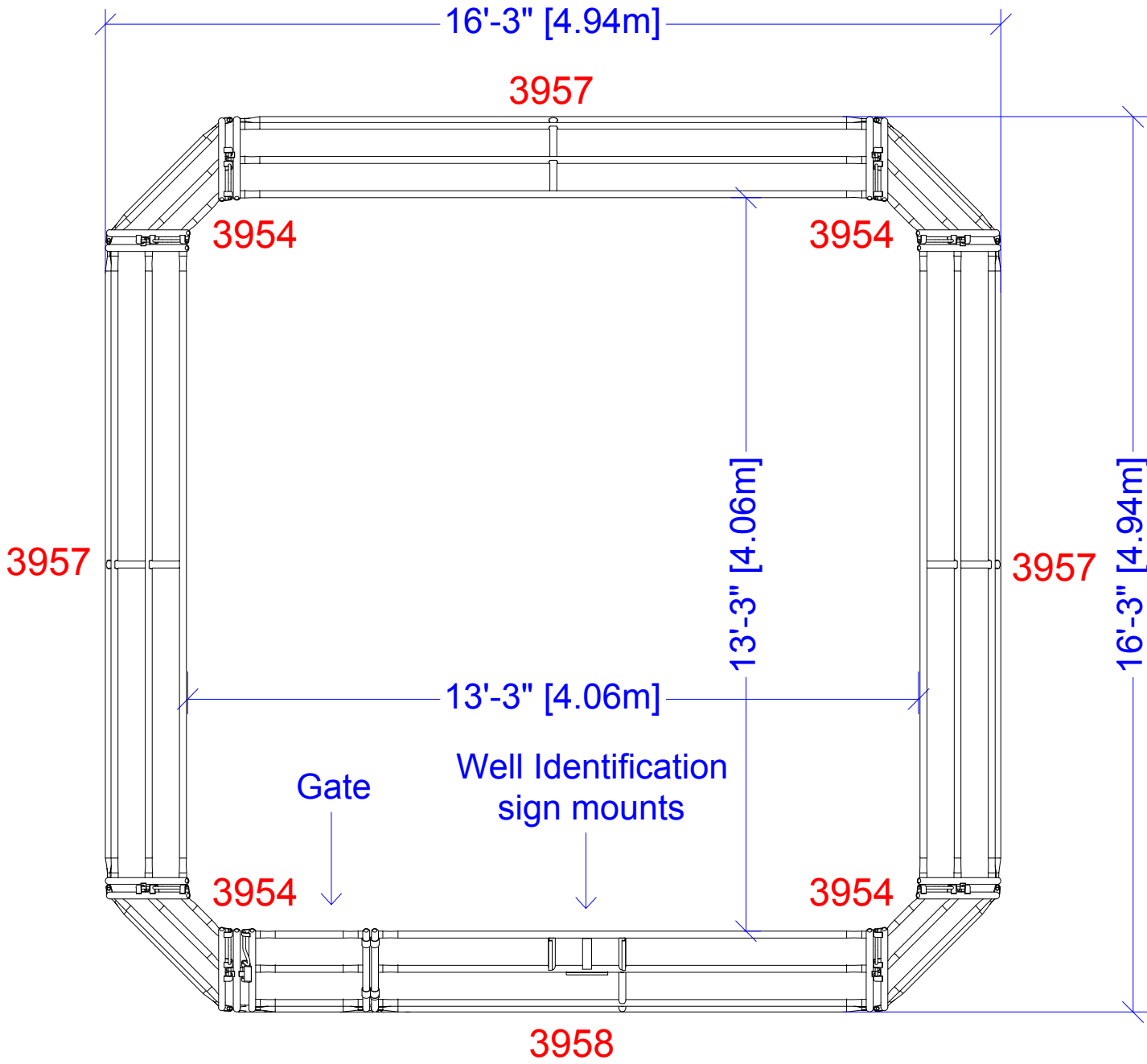
13'-3" x 13'-3" Well fence Enclosure
